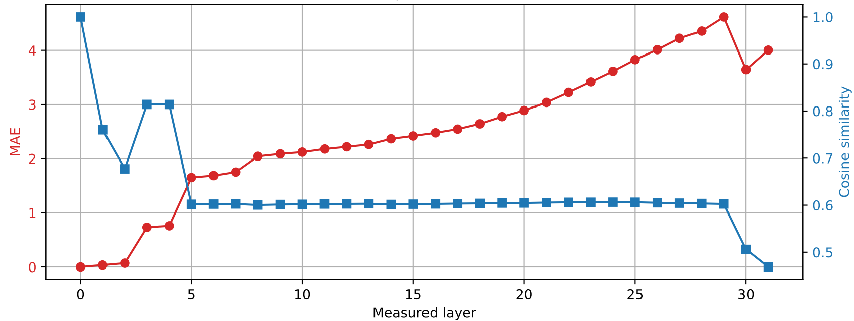
Phi-3-mini-4k-instruct | Prompt 0 Spared layer 24 | Hybrid vs unquantized
