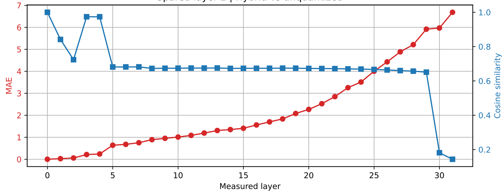
Phi-3-mini-4k-instruct | Prompt 1 Spared layer 2 | Hybrid vs unquantized
