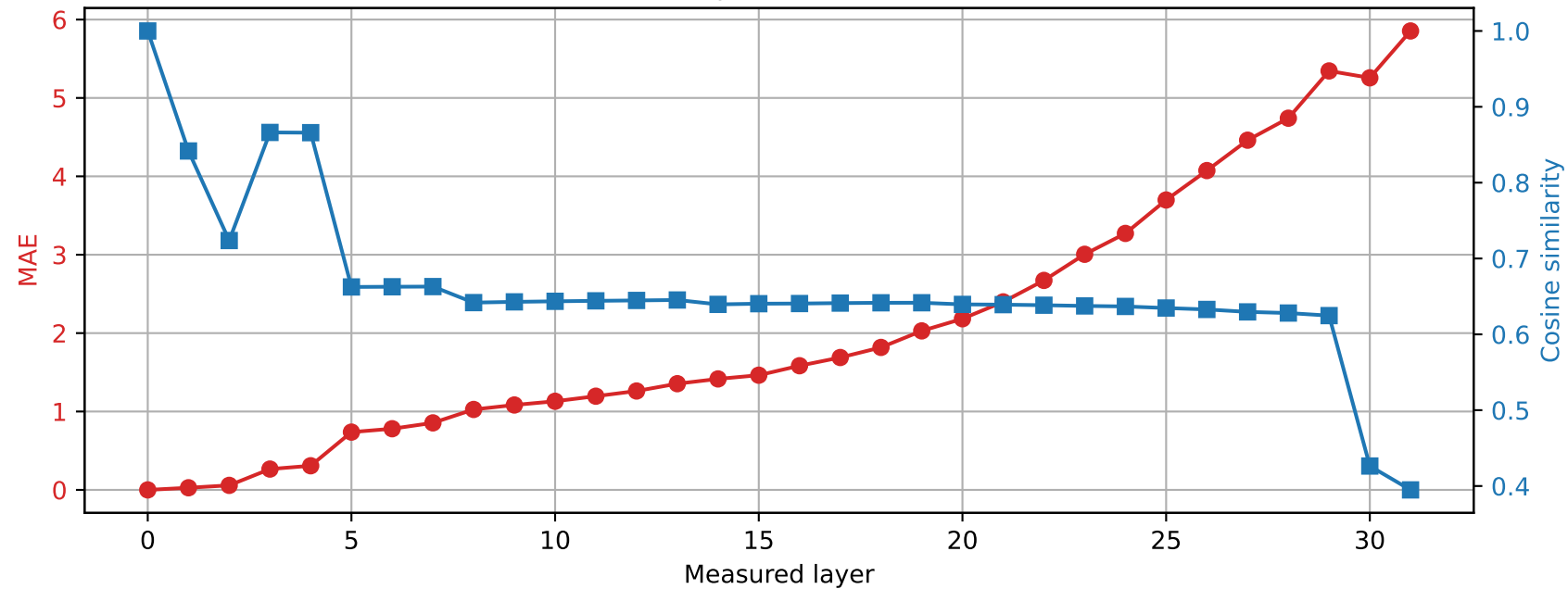
Phi-3-mini-4k-instruct | Prompt 1 Spared layer 3 | Hybrid vs unquantized
