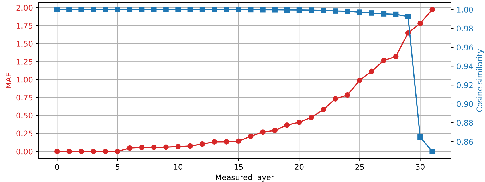
Phi-3-mini-4k-instruct | Prompt 1 Spared layer 5 | Hybrid vs quantized
