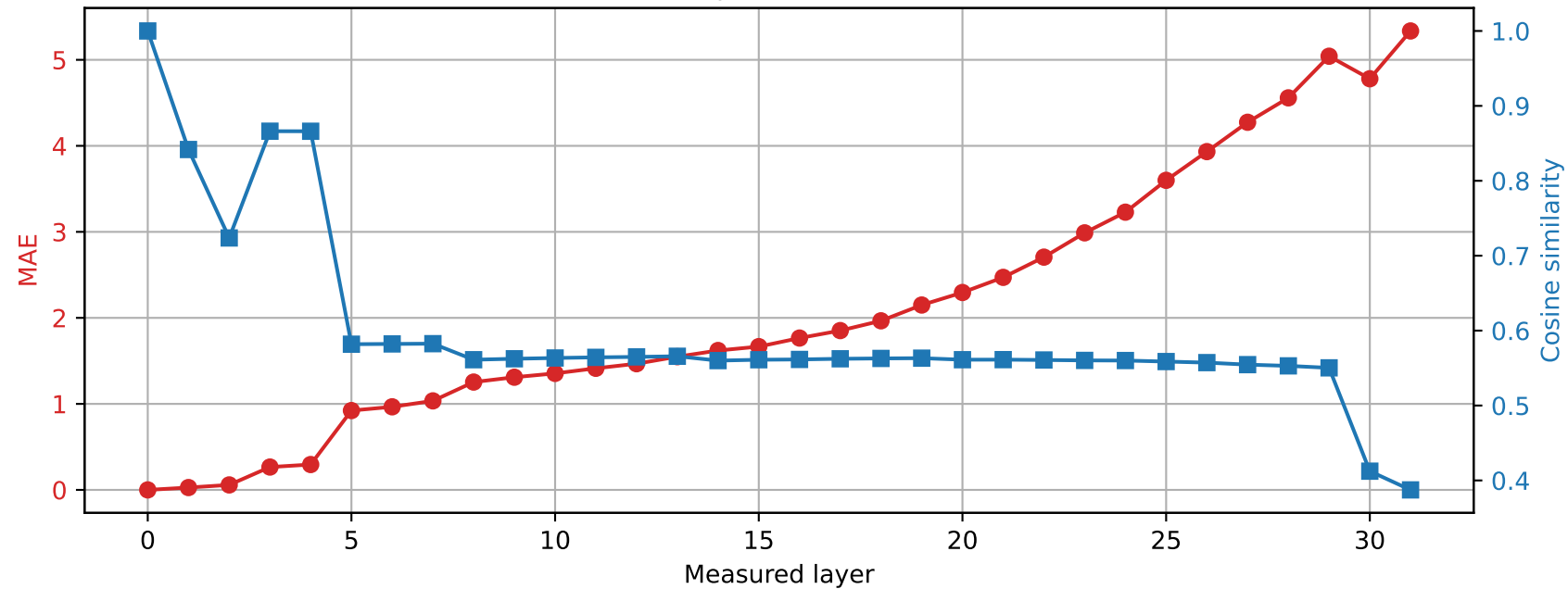
Phi-3-mini-4k-instruct | Prompt 1 Spared layer 5 | Hybrid vs unquantized
