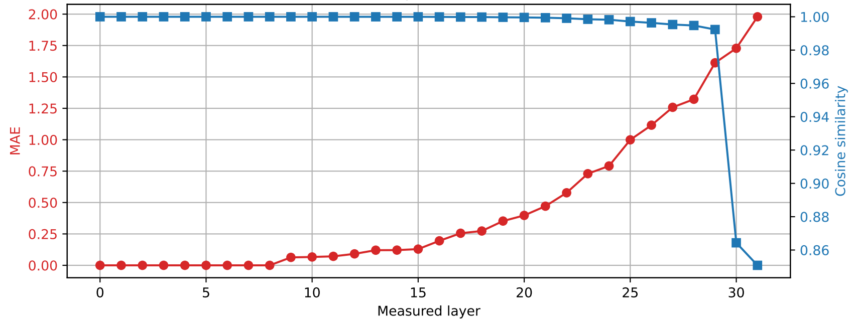
Phi-3-mini-4k-instruct | Prompt 1 Spared layer 8 | Hybrid vs quantized
