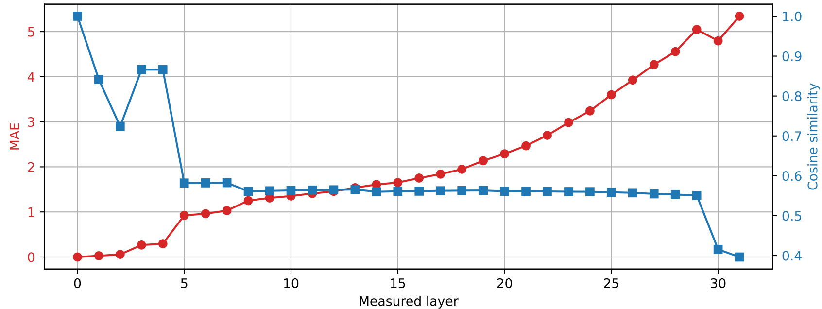
Phi-3-mini-4k-instruct | Prompt 1 Spared layer 8 | Hybrid vs unquantized
