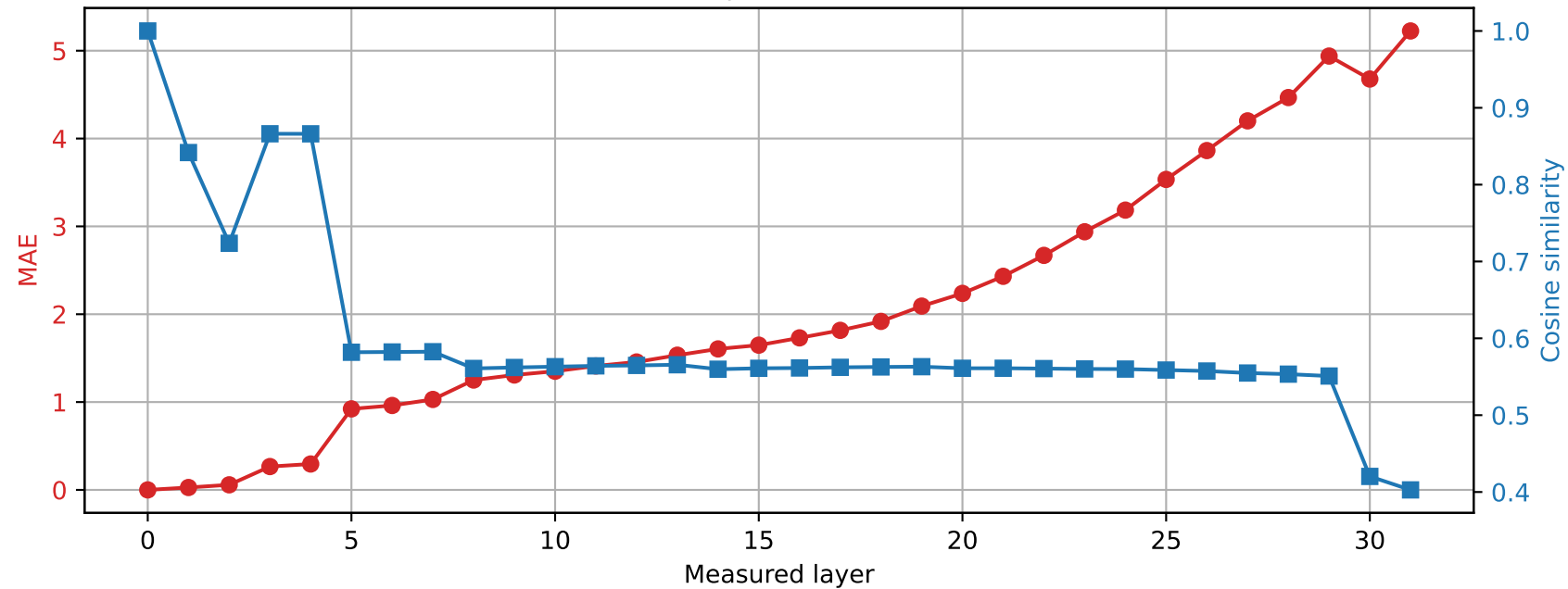
Phi-3-mini-4k-instruct | Prompt 1 Spared layer 10 | Hybrid vs unquantized
