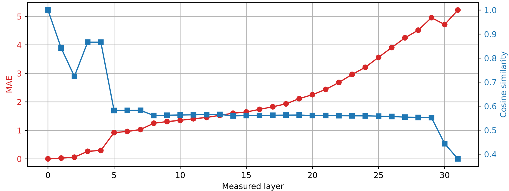
Phi-3-mini-4k-instruct | Prompt 1 Spared layer 28 | Hybrid vs unquantized
