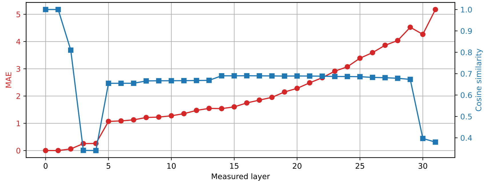
Phi-3-mini-4k-instruct | Prompt 2 Spared layer 1 | Hybrid vs quantized
