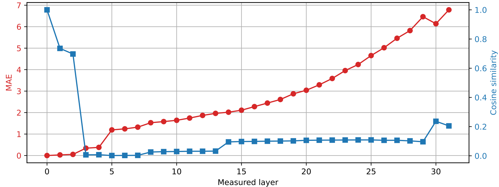
Phi-3-mini-4k-instruct | Prompt 2 Spared layer 19 | Hybrid vs unquantized
