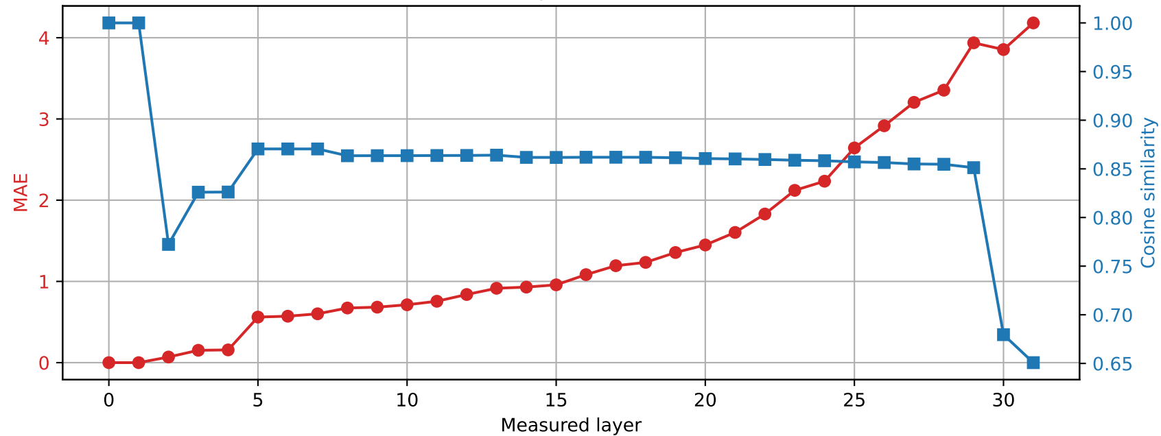
Phi-3-mini-4k-instruct | Prompt 3 Spared layer 1 | Hybrid vs quantized
