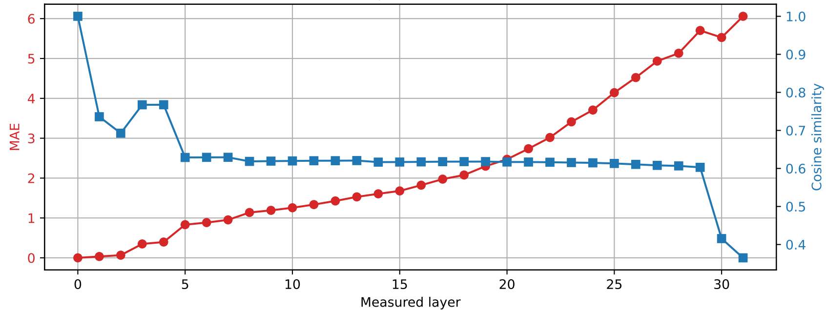
Phi-3-mini-4k-instruct | Prompt 3 Spared layer 3 | Hybrid vs unquantized
