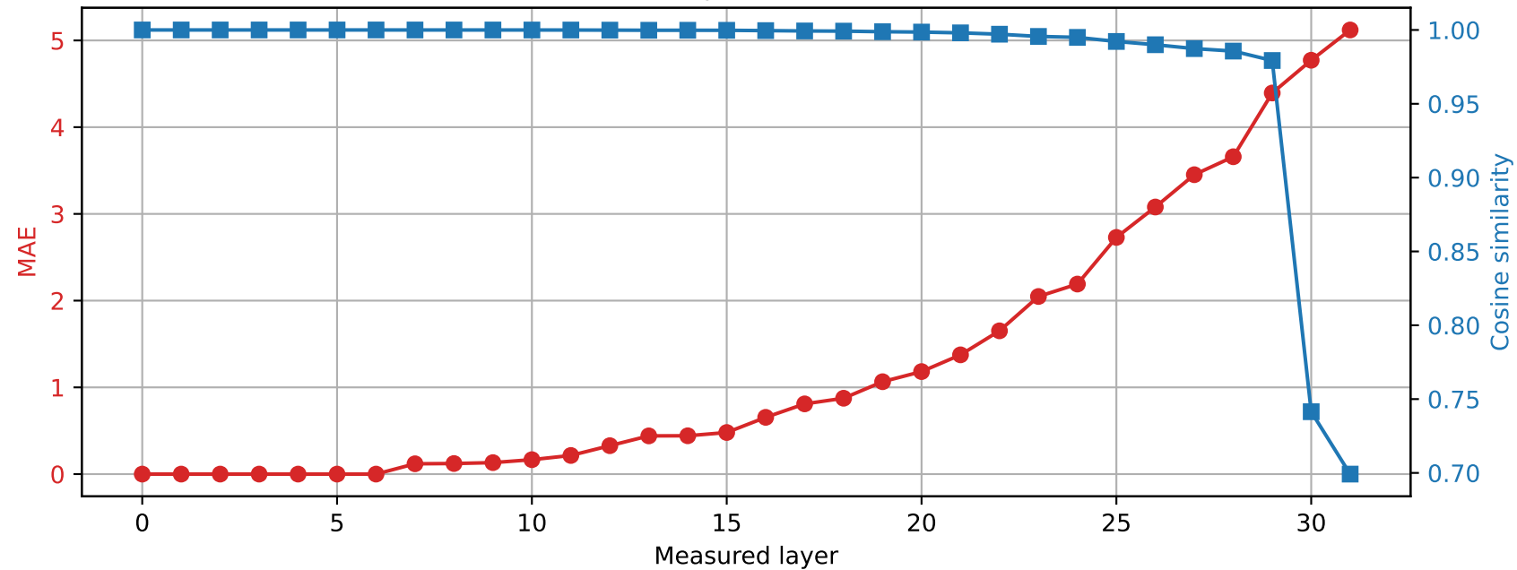
Phi-3-mini-4k-instruct | Prompt 3 Spared layer 6 | Hybrid vs quantized
