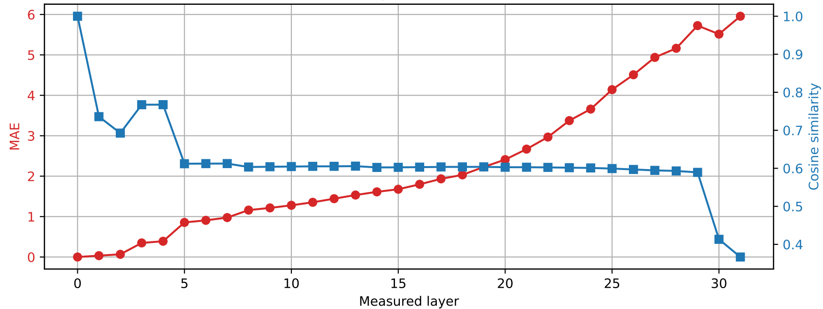
Phi-3-mini-4k-instruct | Prompt 3 Spared layer 12 | Hybrid vs unquantized
