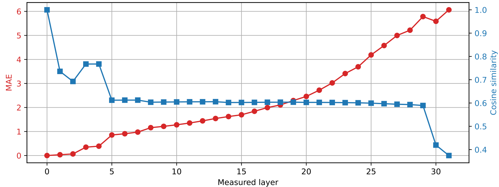
Phi-3-mini-4k-instruct | Prompt 3 Spared layer 17 | Hybrid vs unquantized
