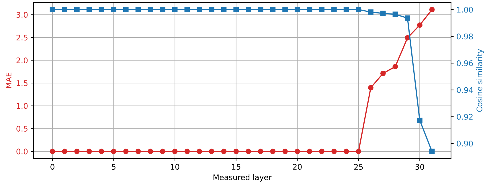
Phi-3-mini-4k-instruct | Prompt 3 Spared layer 25 | Hybrid vs quantized
