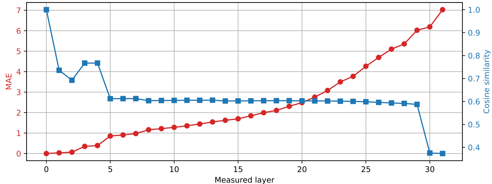
Phi-3-mini-4k-instruct | Prompt 3 Spared layer 29 | Hybrid vs unquantized
