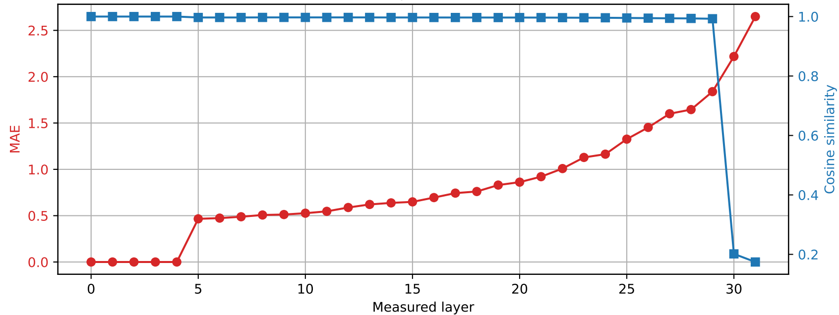
Phi-3-mini-4k-instruct | Prompt 4 Spared layer 4 | Hybrid vs quantized
