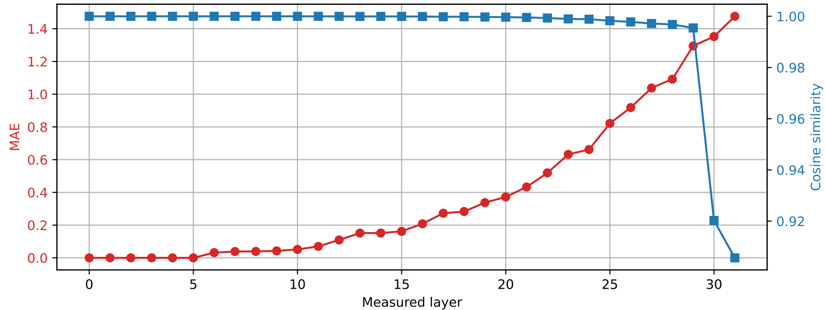
Phi-3-mini-4k-instruct | Prompt 4 Spared layer 5 | Hybrid vs quantized
