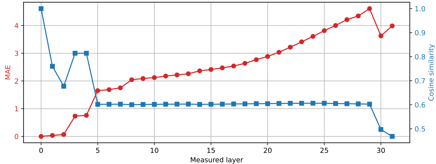
Phi-3-mini-4k-instruct | Prompt 0 Spared layer 9 | Hybrid vs unquantized
