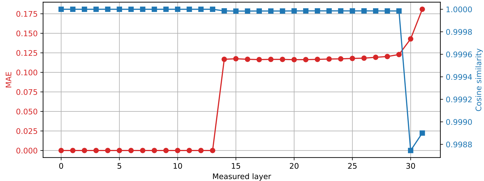
Phi-3-mini-4k-instruct | Prompt 0 Spared layer 13 | Hybrid vs quantized
