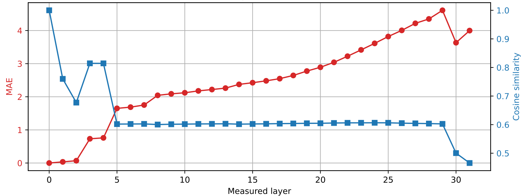
Phi-3-mini-4k-instruct | Prompt 0 Spared layer 13 | Hybrid vs unquantized
