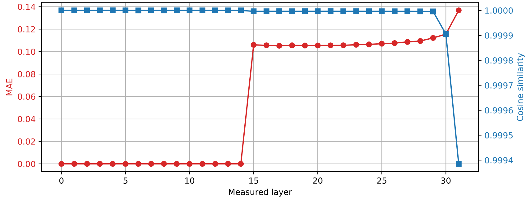
Phi-3-mini-4k-instruct | Prompt 0 Spared layer 14 | Hybrid vs quantized
