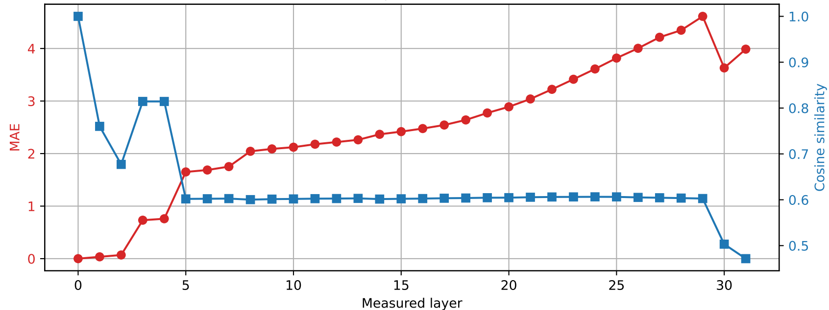
Phi-3-mini-4k-instruct | Prompt 0 Spared layer 16 | Hybrid vs unquantized
