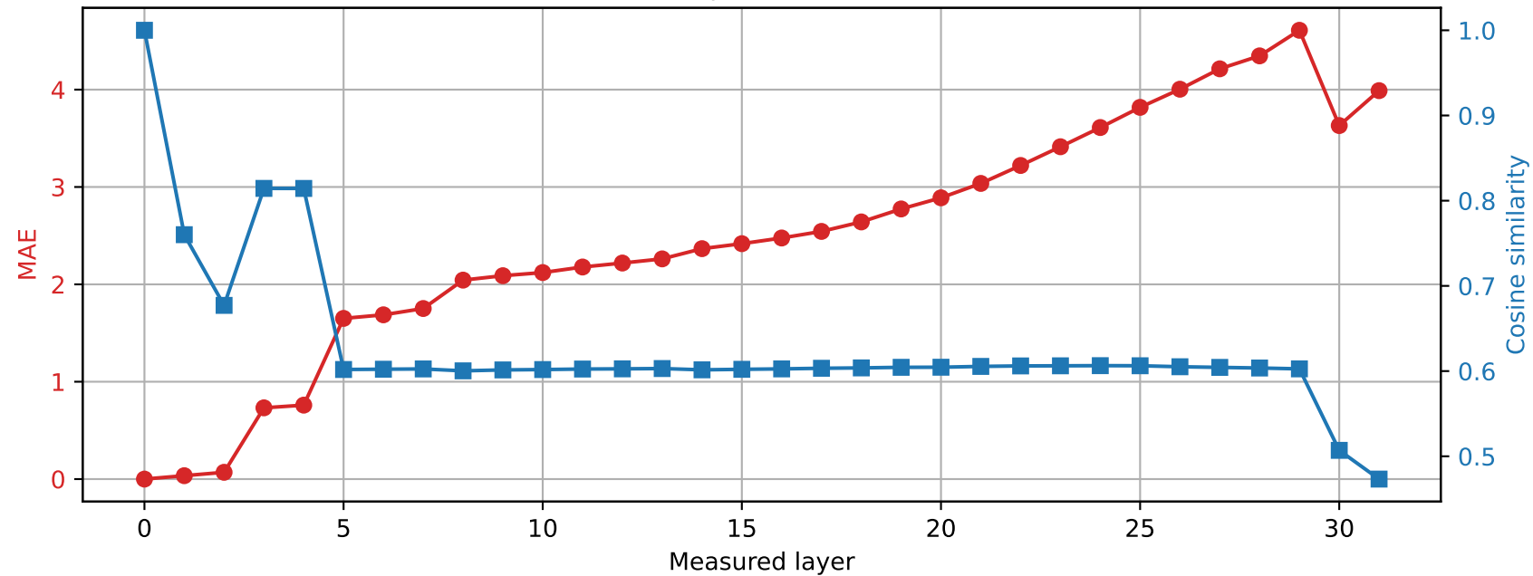
Phi-3-mini-4k-instruct | Prompt 0 Spared layer 20 | Hybrid vs unquantized
