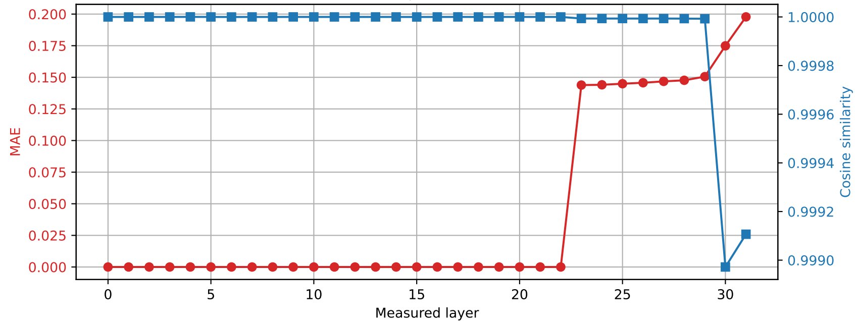
Phi-3-mini-4k-instruct | Prompt 0 Spared layer 22 | Hybrid vs quantized
