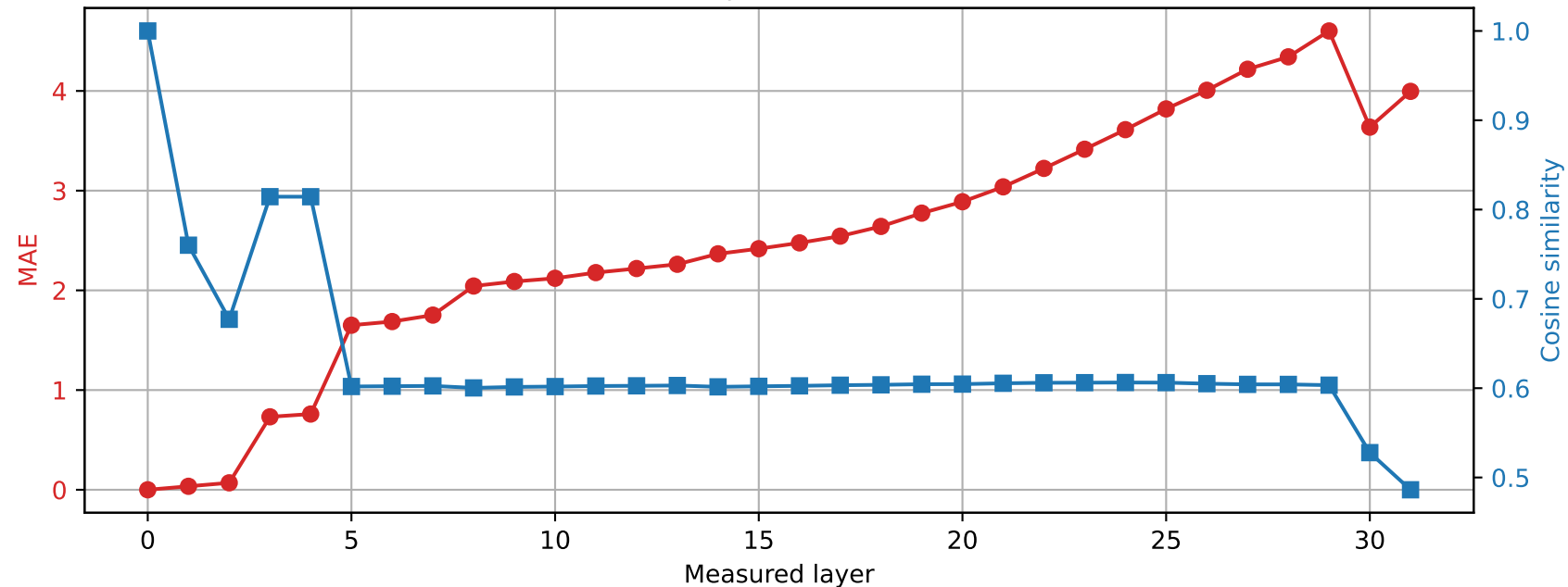
Phi-3-mini-4k-instruct | Prompt 0 Spared layer 27 | Hybrid vs unquantized
