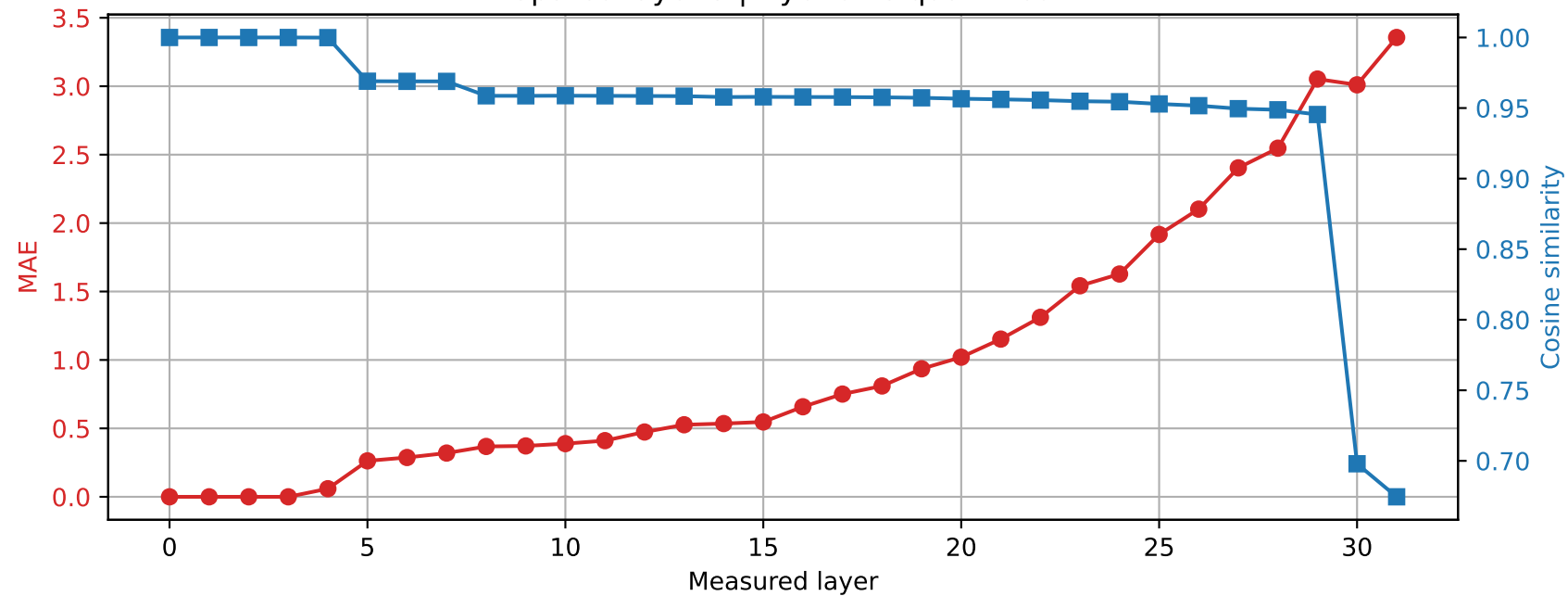
Phi-3-mini-4k-instruct | Prompt 1 Spared layer 3 | Hybrid vs quantized
