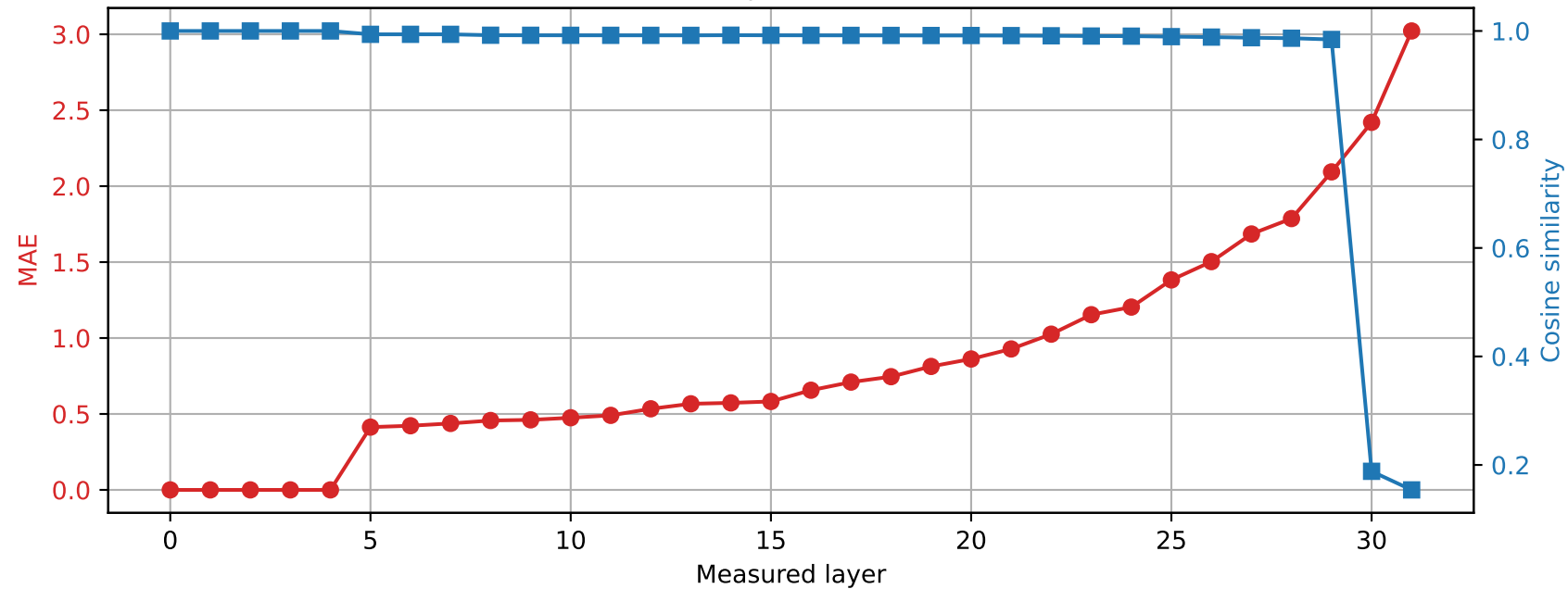
Phi-3-mini-4k-instruct | Prompt 1 Spared layer 4 | Hybrid vs quantized
