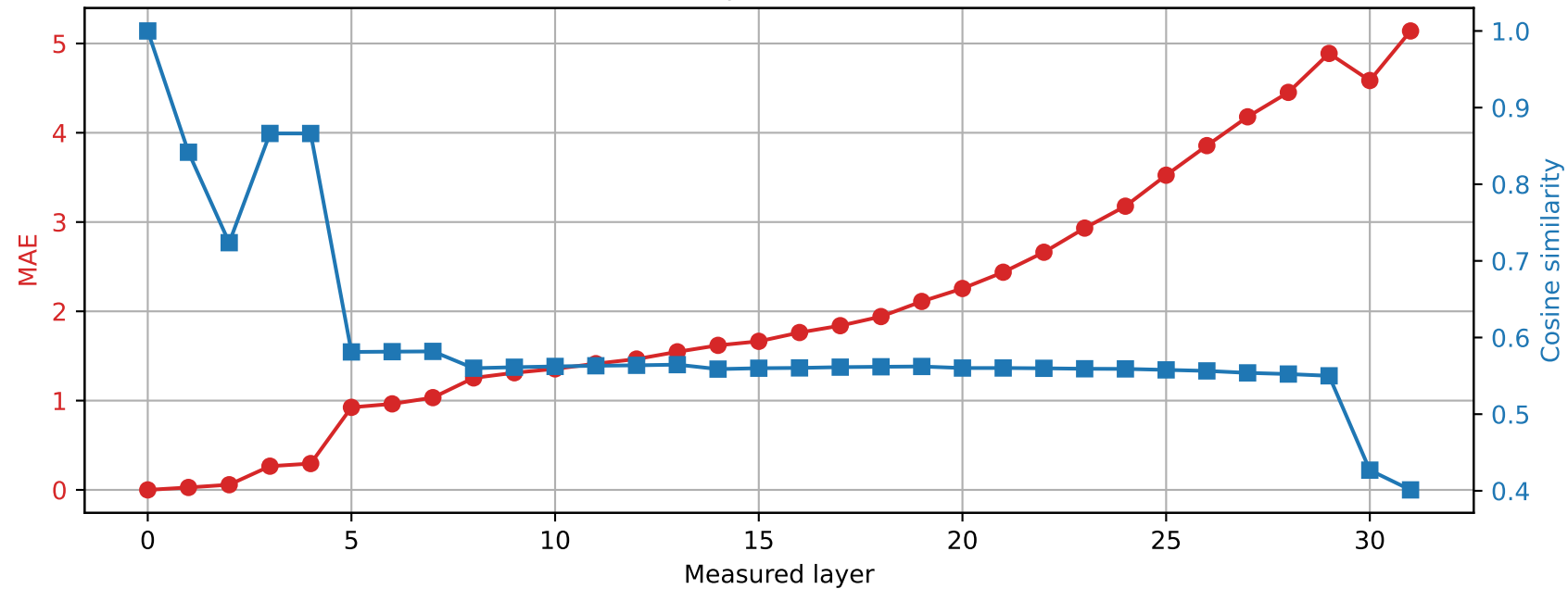
Phi-3-mini-4k-instruct | Prompt 1 Spared layer 16 | Hybrid vs unquantized
