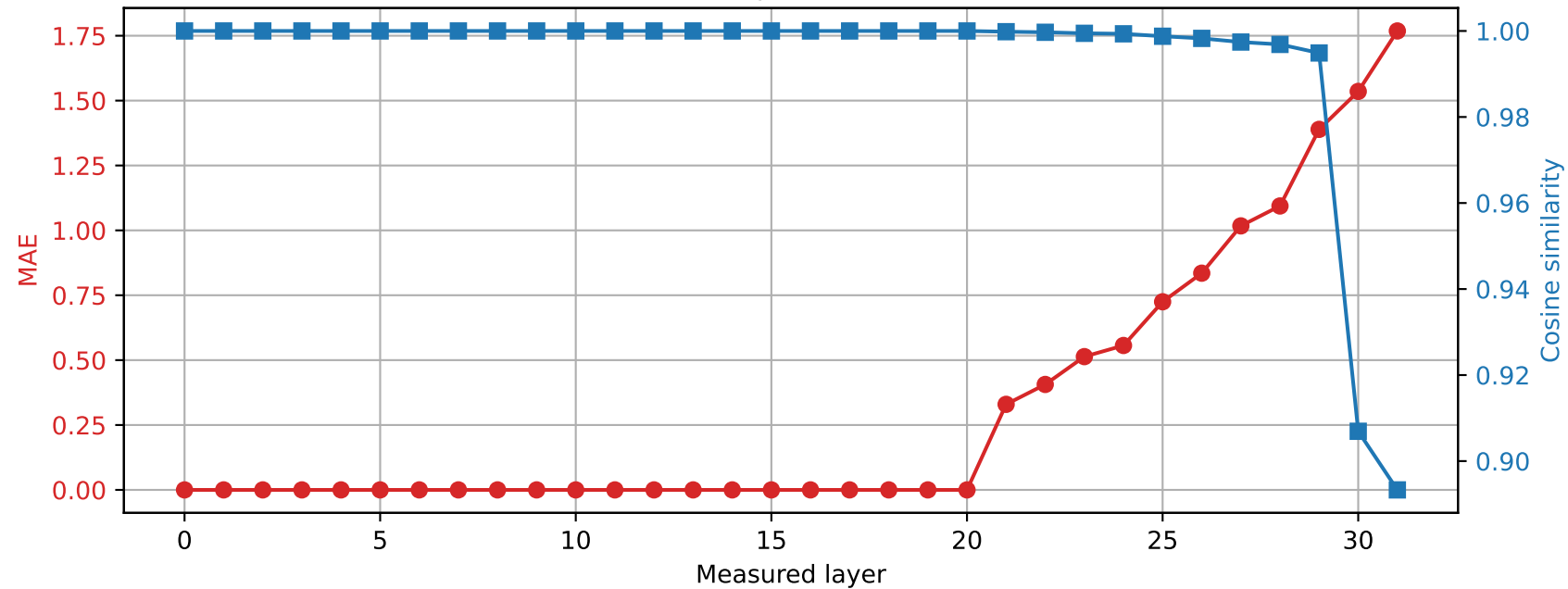
Phi-3-mini-4k-instruct | Prompt 1 Spared layer 20 | Hybrid vs quantized
