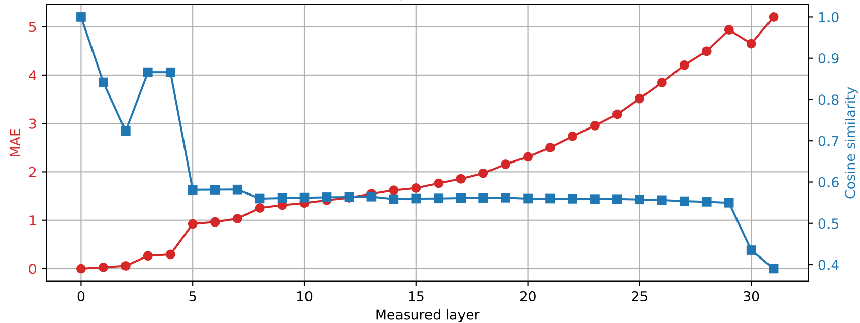
Phi-3-mini-4k-instruct | Prompt 1 Spared layer 22 | Hybrid vs unquantized
