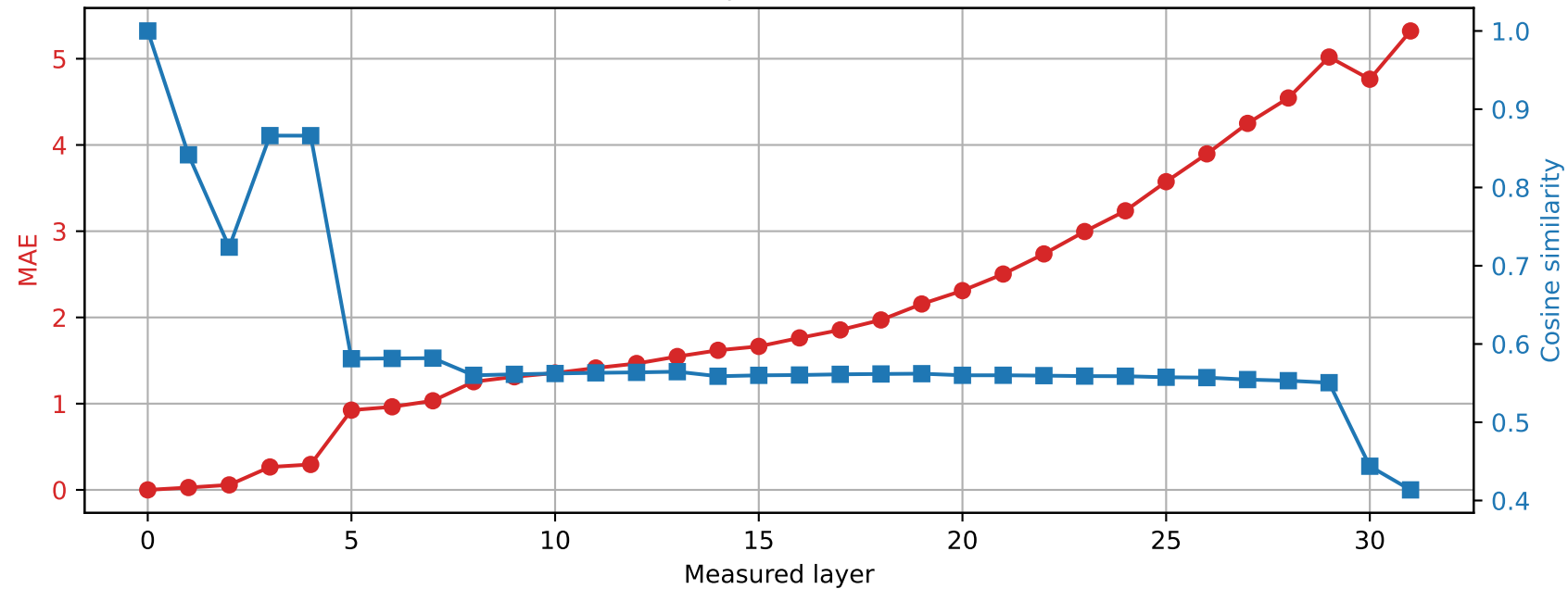
Phi-3-mini-4k-instruct | Prompt 1 Spared layer 25 | Hybrid vs unquantized
