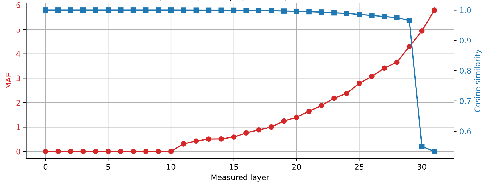
Phi-3-mini-4k-instruct | Prompt 2 Spared layer 10 | Hybrid vs quantized
