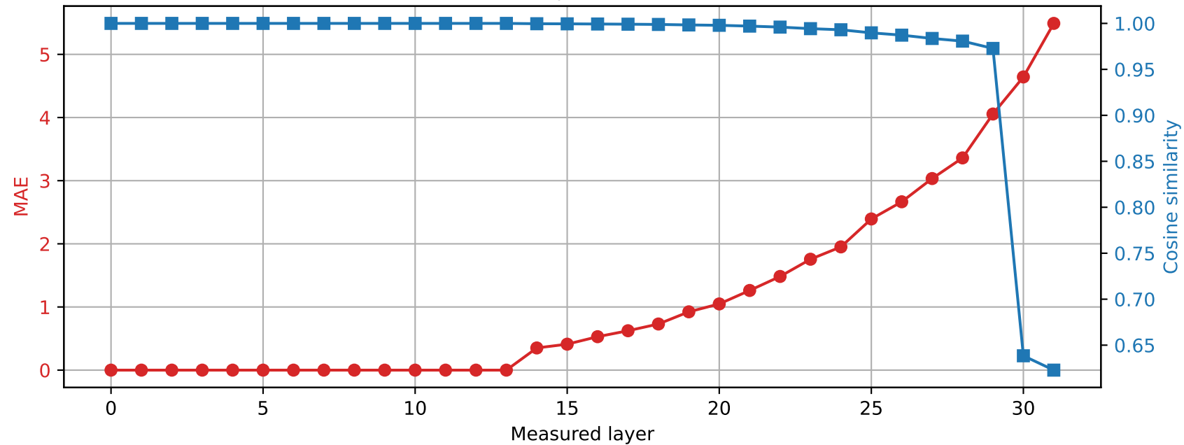
Phi-3-mini-4k-instruct | Prompt 2 Spared layer 13 | Hybrid vs quantized
