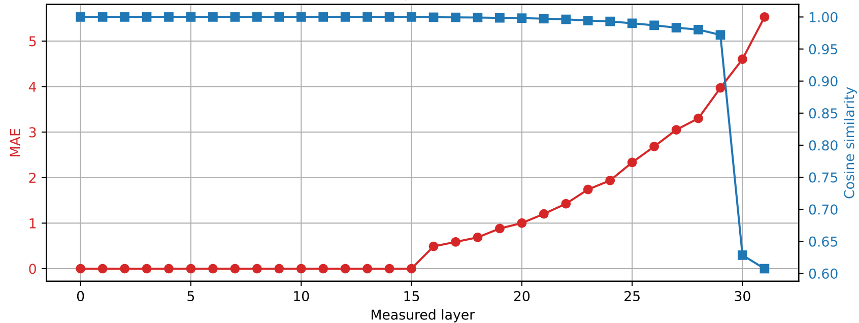
Phi-3-mini-4k-instruct | Prompt 2 Spared layer 15 | Hybrid vs quantized
