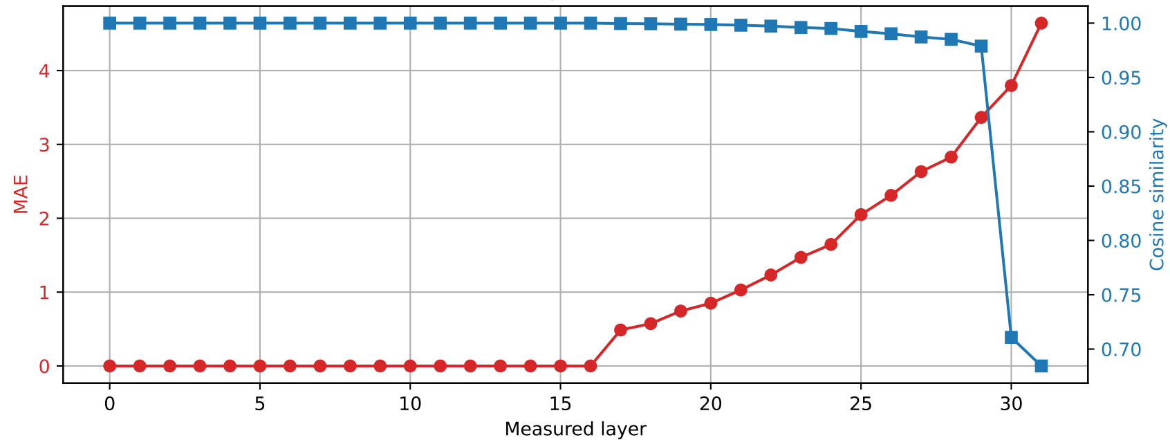
Phi-3-mini-4k-instruct | Prompt 2 Spared layer 16 | Hybrid vs quantized
