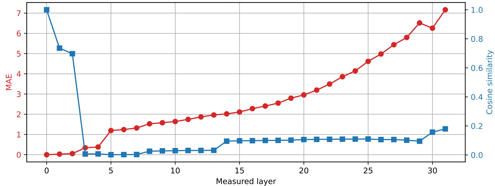
Phi-3-mini-4k-instruct | Prompt 2 Spared layer 16 | Hybrid vs unquantized
