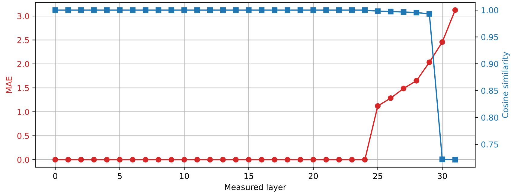
Phi-3-mini-4k-instruct | Prompt 2 Spared layer 24 | Hybrid vs quantized
