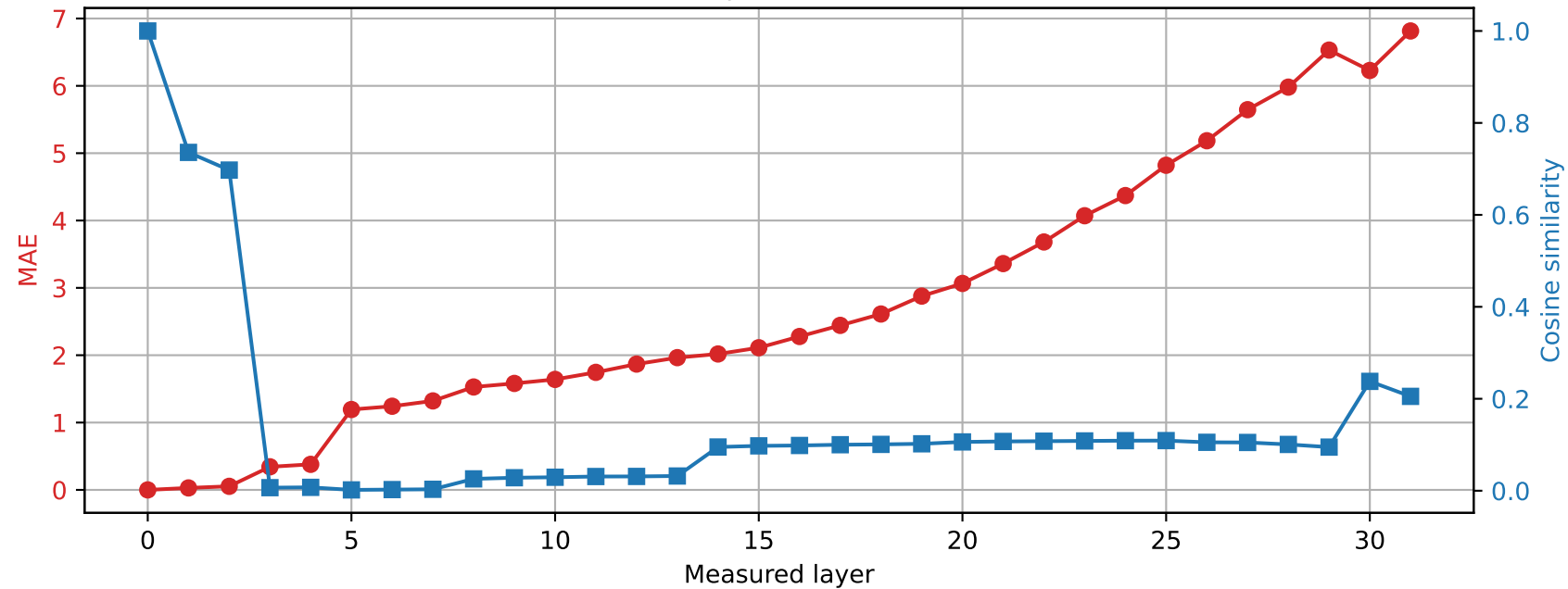
Phi-3-mini-4k-instruct | Prompt 2 Spared layer 28 | Hybrid vs unquantized
