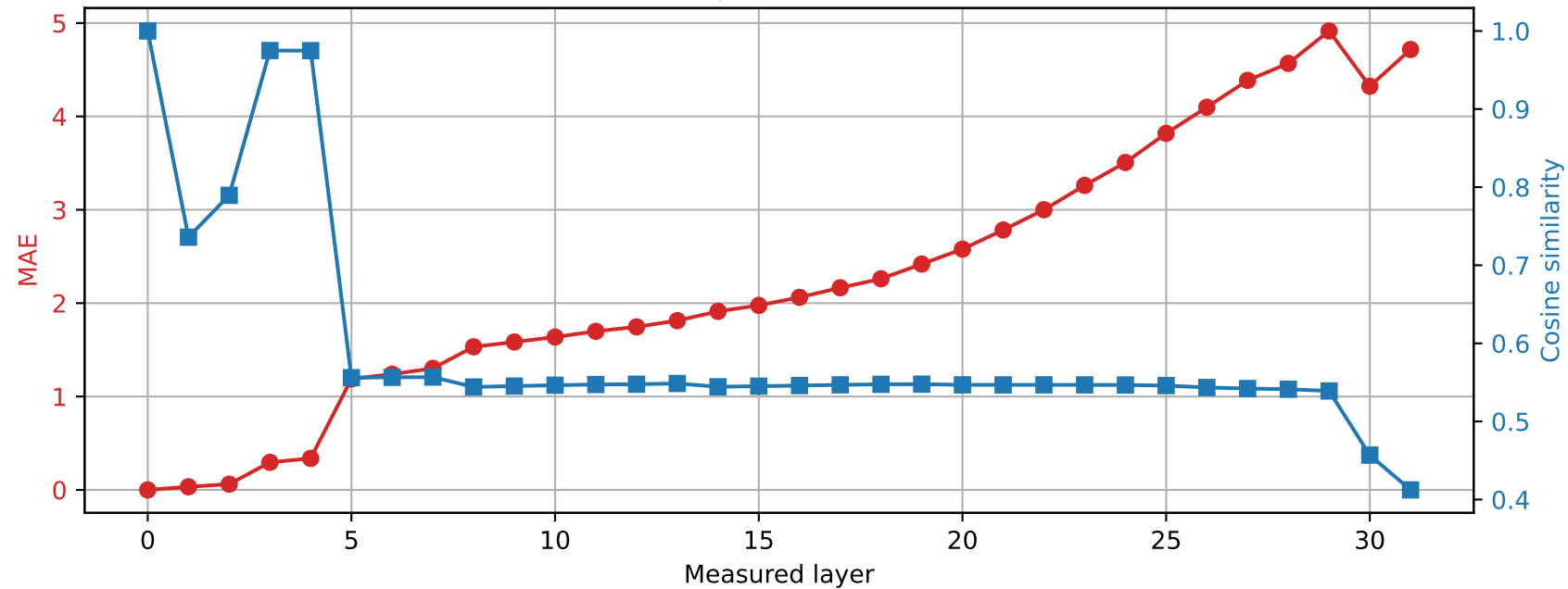
Phi-3-mini-4k-instruct | Prompt 3 Spared layer 1 | Hybrid vs unquantized
