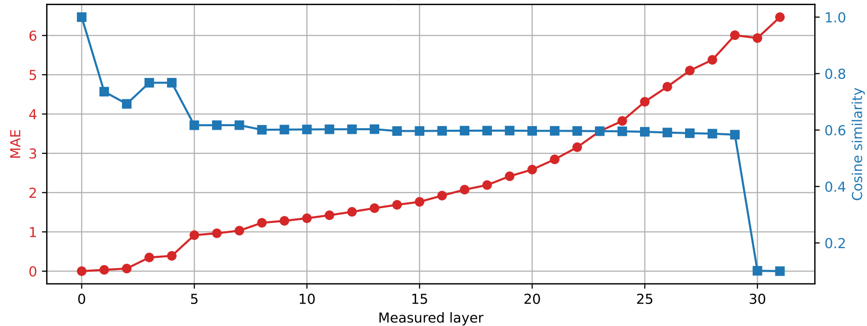
Phi-3-mini-4k-instruct | Prompt 3 Spared layer 4 | Hybrid vs unquantized
