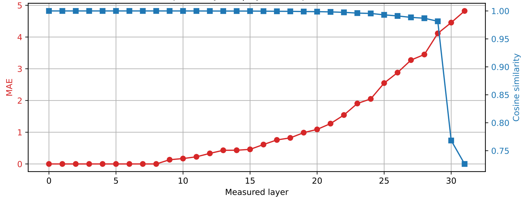
Phi-3-mini-4k-instruct | Prompt 3 Spared layer 8 | Hybrid vs quantized
