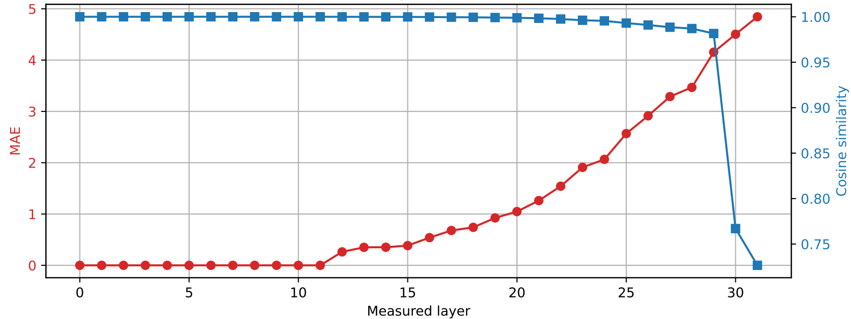
Phi-3-mini-4k-instruct | Prompt 3 Spared layer 11 | Hybrid vs quantized
