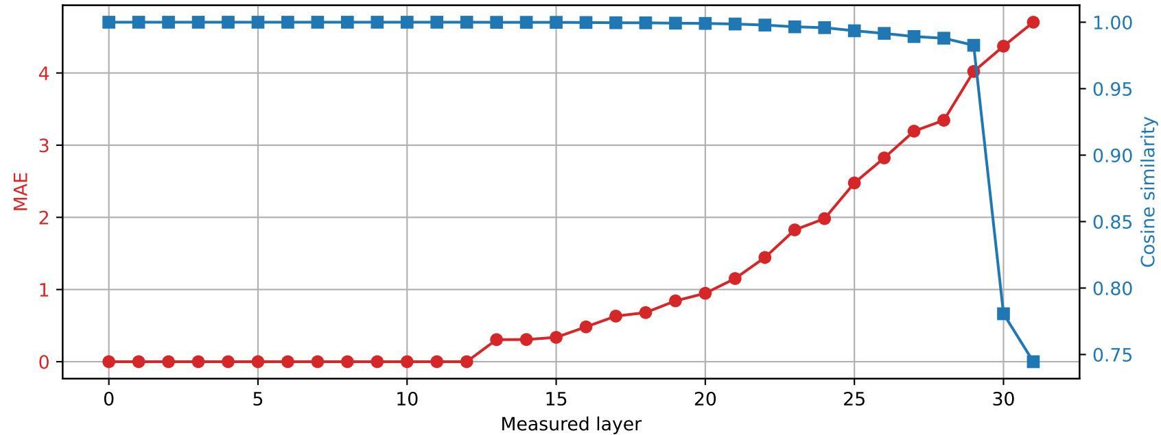
Phi-3-mini-4k-instruct | Prompt 3 Spared layer 12 | Hybrid vs quantized
