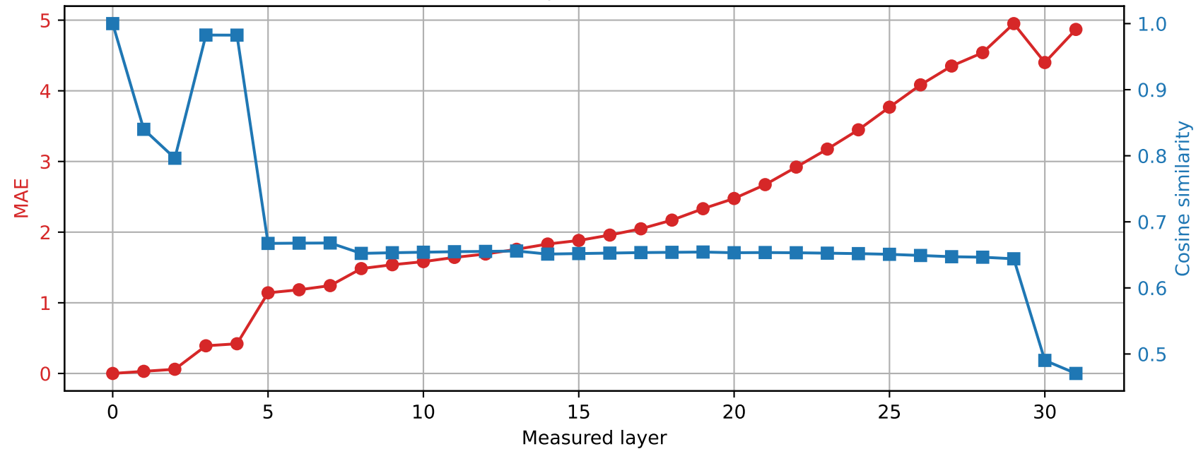
Phi-3-mini-4k-instruct | Prompt 4 Spared layer 6 | Hybrid vs unquantized
