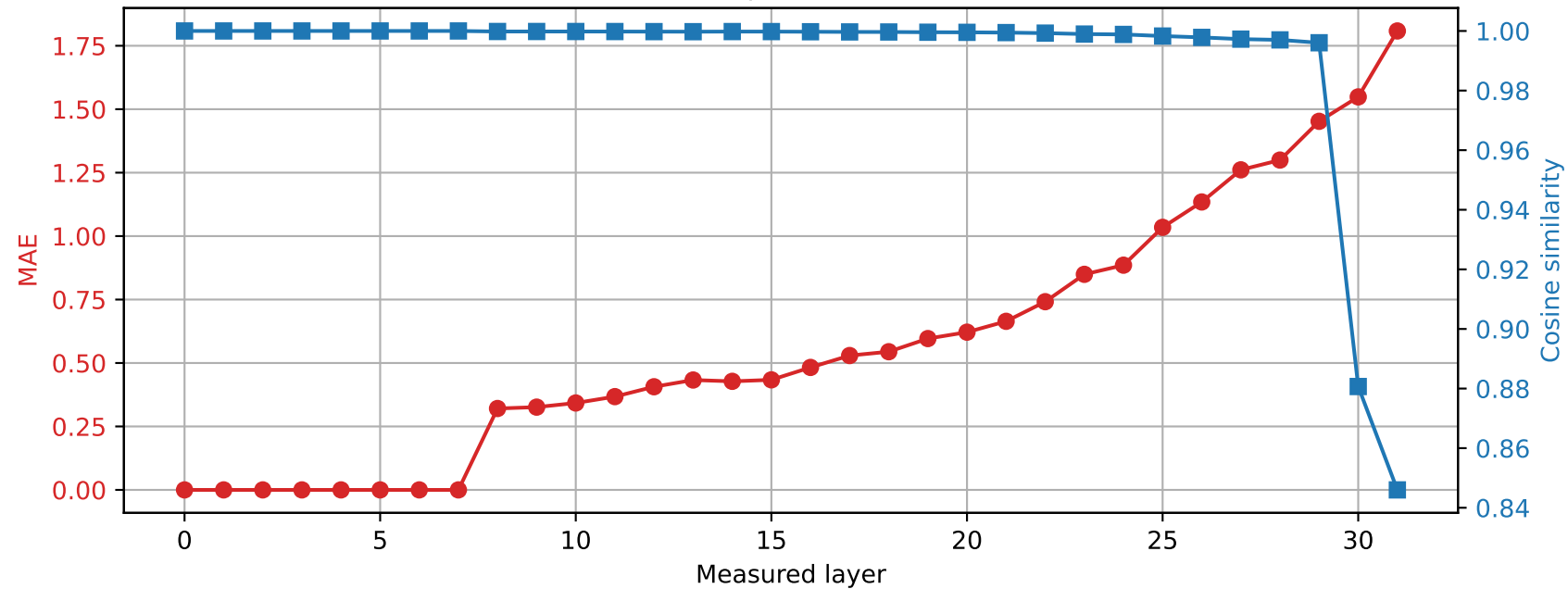
Phi-3-mini-4k-instruct | Prompt 4 Spared layer 7 | Hybrid vs quantized
