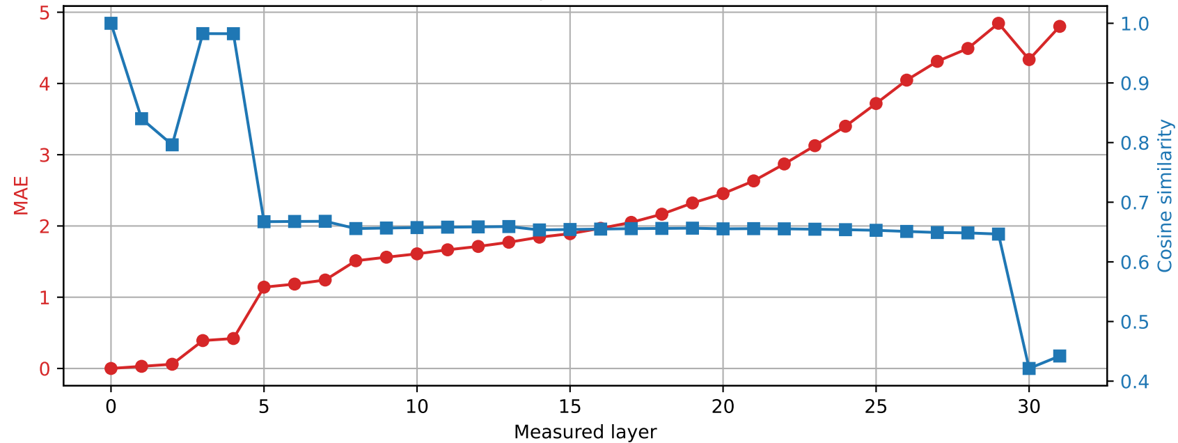
Phi-3-mini-4k-instruct | Prompt 4 Spared layer 7 | Hybrid vs unquantized
