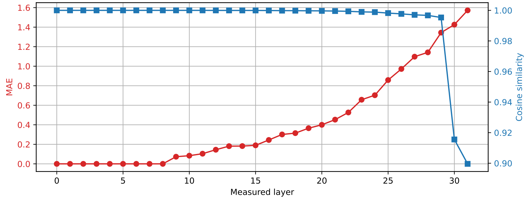
Phi-3-mini-4k-instruct | Prompt 4 Spared layer 8 | Hybrid vs quantized
